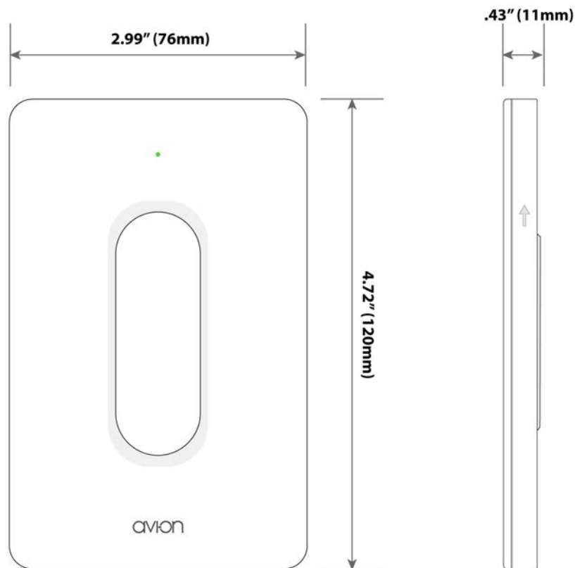
Figure 1. Avi-on Movable Switch Dimensions
